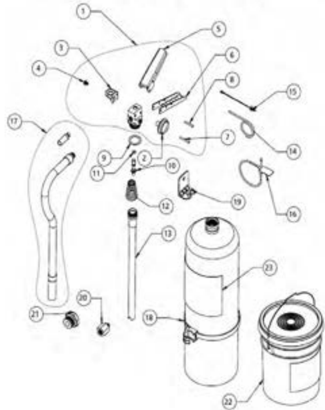
BADGER EXTRA STORED PRESSURE DRY CHEMICAL PORTABLE EXTINGUISHER DIAGRAM (BRASS VALVE)
